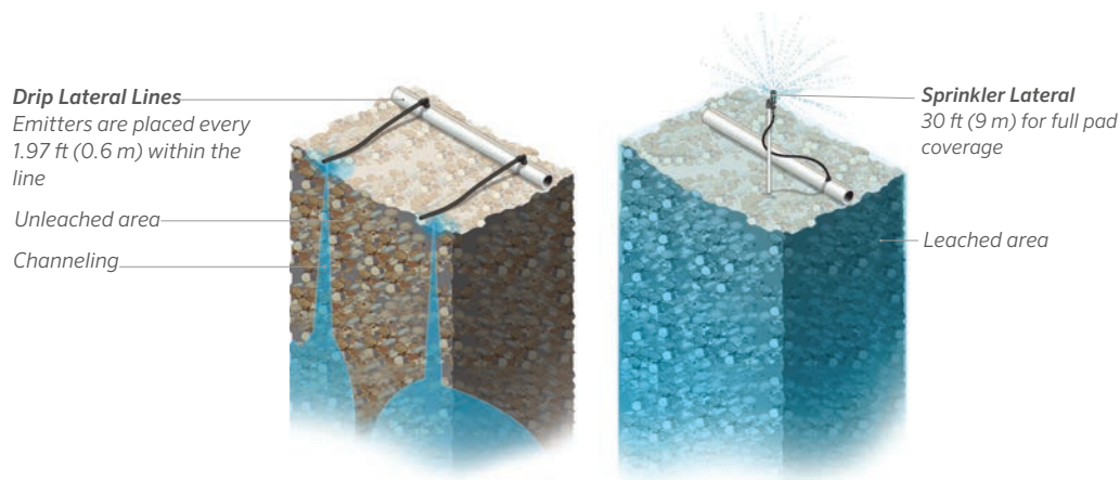
Drip systems depend on the source point application of the solution, which promotes channeling. With a minimal lateral movement of the applied solution, drip systems have a challenge achieving the desired application rate.
